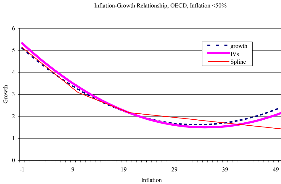
Figure 6: Quadratic Specification
