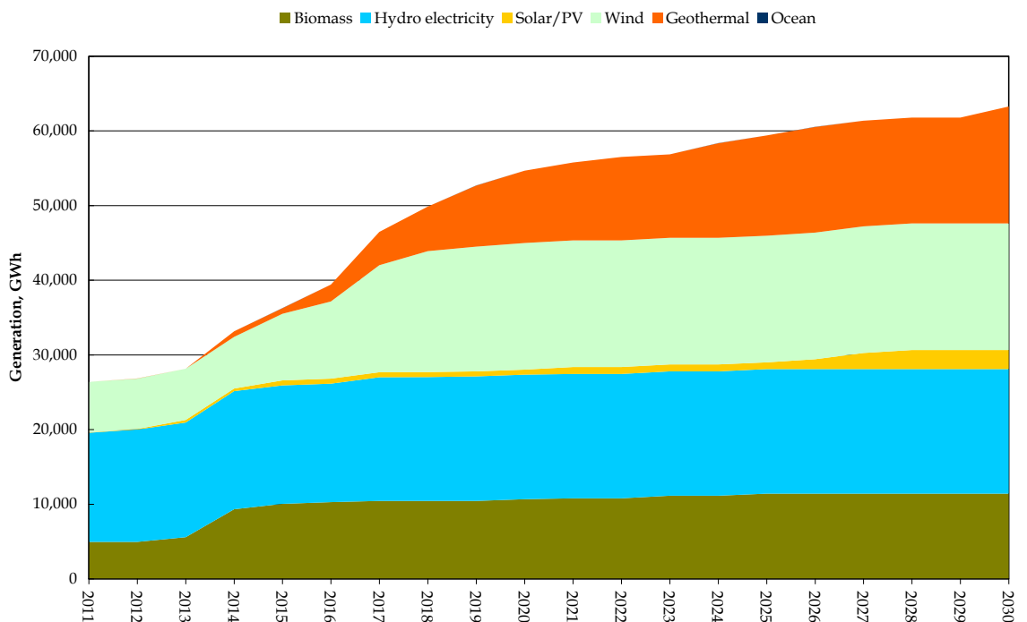
Figure 3-24: Generation mix (large scale plant) – LRET design
